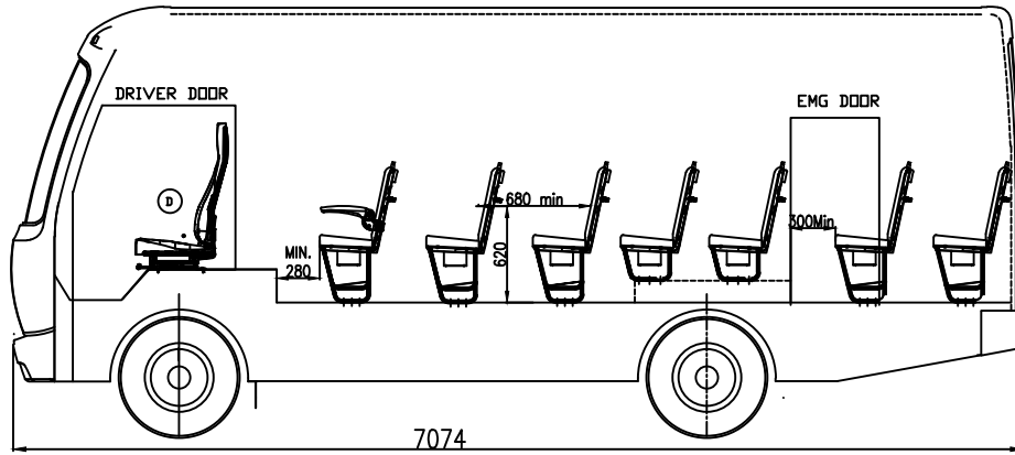
RH SIDE
